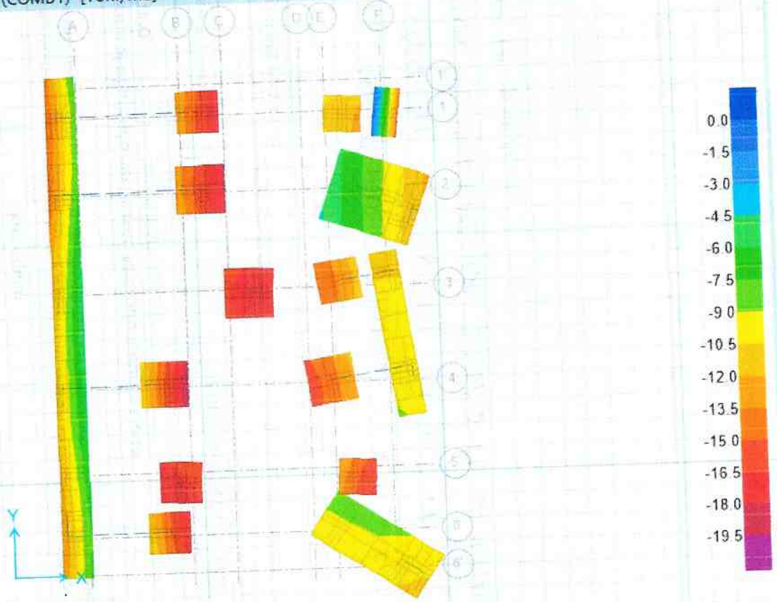
Pressure Diagram - (COMB1) [Tonf/m2]
